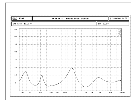
Impedance Curve
