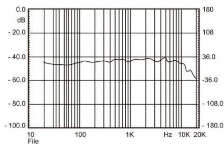
Frequency Response
