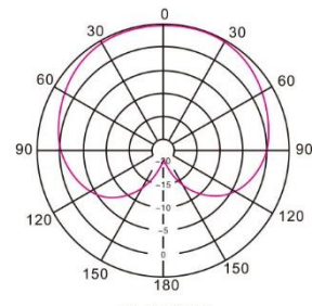
Polar Pattern
