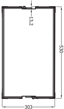
SECTION C-C
