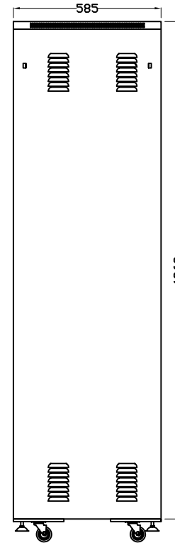
END VIEW
